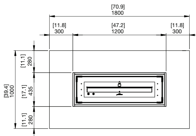
Line drawings show concrete models without a Fire Screen. Refer to the Fire Screen model specifications for dimensions.
